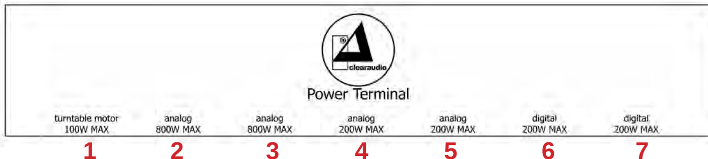
Pic. 2: Explanation of connections
